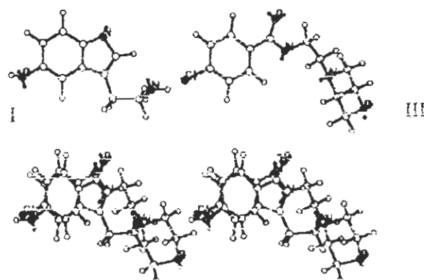
Fig. 2. Stereoview of the superimposition of two gauche forms of serotonin (I) and moclobemide (III).
