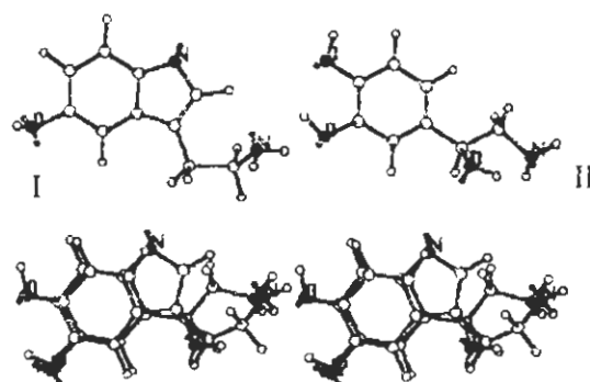
Fig. 1. Stereoview of the superimposition of the gauche form of serotonin (I) and the extended form of norepinephrine (II).
